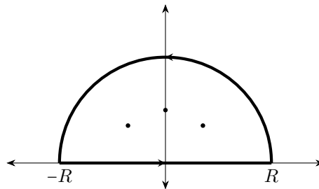
Figure 8: Contour in the upper half-plane, with the three points denoting the three simple poles of f(z) in the upper half-plane.
