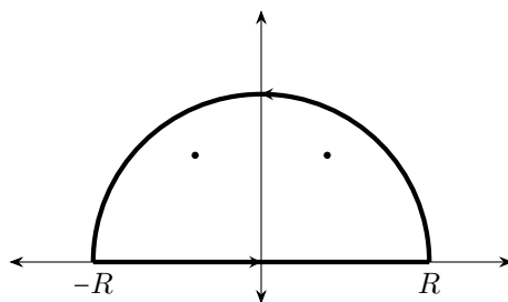
Figure 7: Contour in the upper half-plane, with the two points denoting the two simple poles of f(z) in the upper half-plane.
